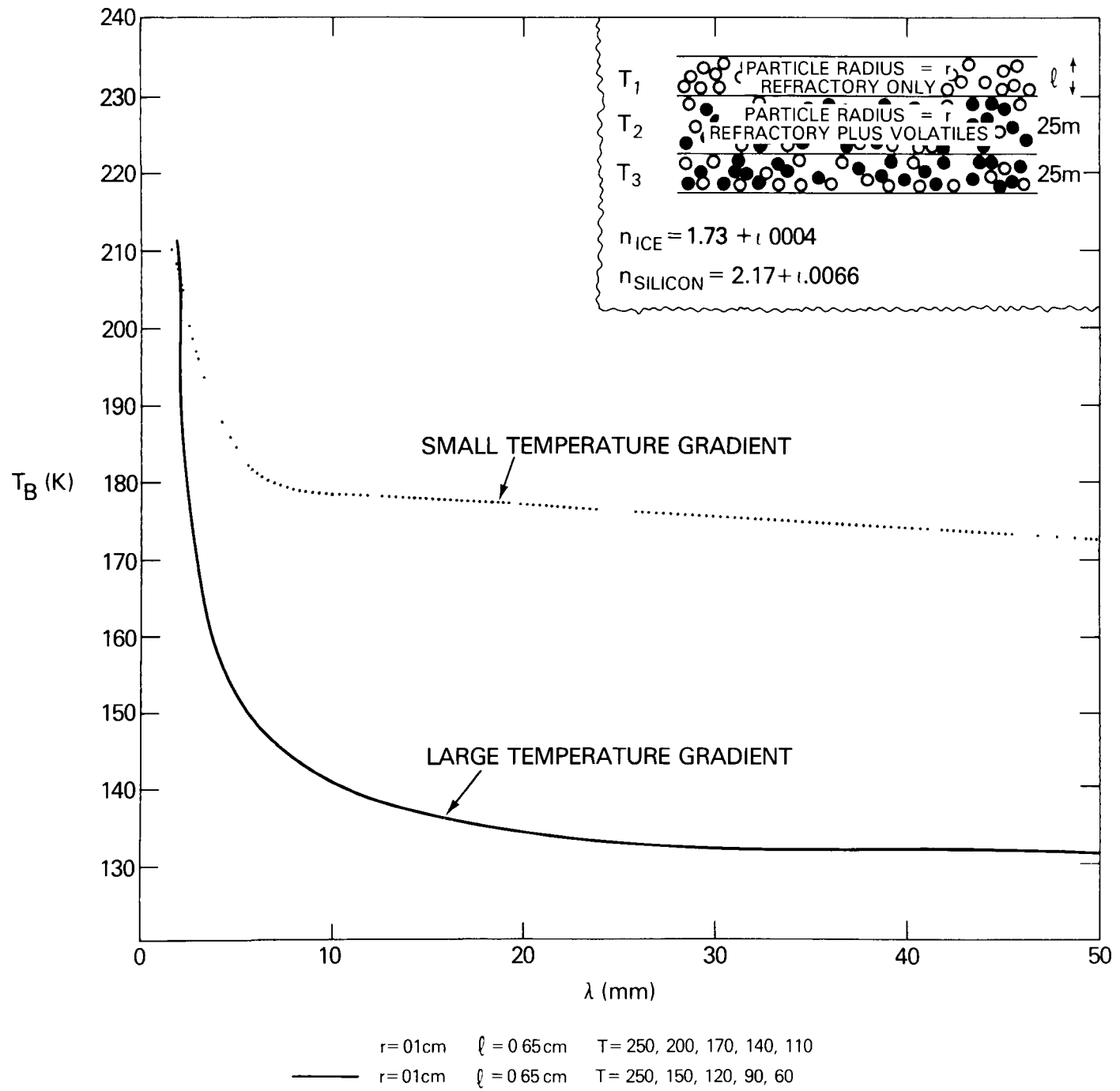
Figure 3. Brightness temperature as a function of wavelength for models with different temperature gradients through the surface crust.
